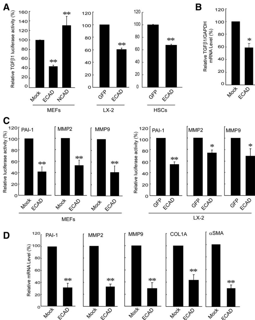
Fig. 2. Effects of ECAD on TGFβ1 and its target gene transactivation. (A) Inhibition of the basal TGFβ1 gene expression by ECAD. MEFs were transfected with a TGFβ1 luciferase construct in combination with the construct encoding for ECAD or NCAD (pCEP4 for mock transfection). LX-2 cells or HSCs were infected with adenoviral GFP or ECAD. The activity of luciferase was normalized by the activity of β-galactosidase. (B) Real-time PCR assays. TGFβ1 mRNA levels were measured in MEFs that had been stably transfected with ECAD. (C) Reporter gene activities. (D) Real-time PCR assays in MEFs stably transfected with ECAD. The data are the means and standard errors of at least three separate experiments (significantly different in comparison with a mock transfection or adenoviral GFP infection: ** P < 0.01 and * P < 0.05 ).
